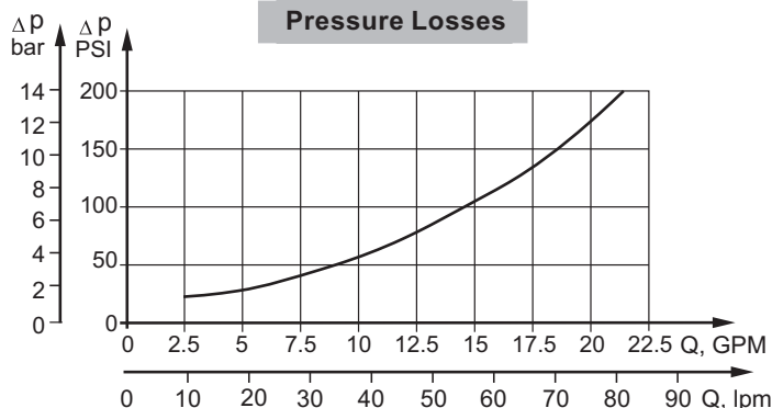
Pressure Losses
