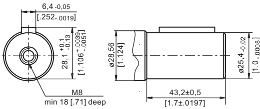
CO - \varnothing 1" straight, Parallel key 1/4 \times 1/4 \times 1 1/4 " BS46 Max. Torque 34 daNm [3010 lb-in]
